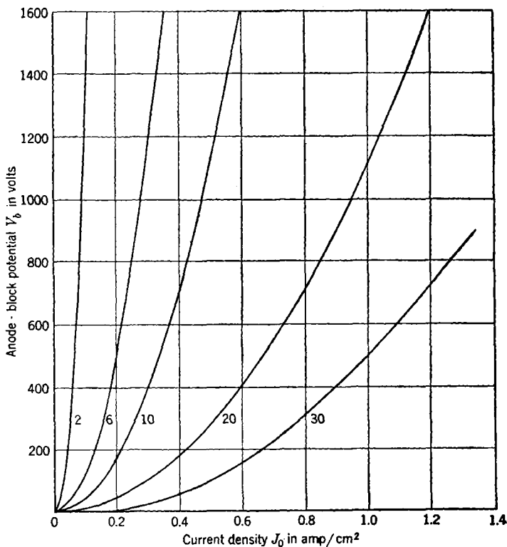
Fig. 15-6.—Anode-block potential V_b as a function of current density J_0 for various values of (D/d)(1 - \beta^2)/p(\nu\Delta\nu/10^4) with (V_b/V_0)^{1/2} = 1.58 .
